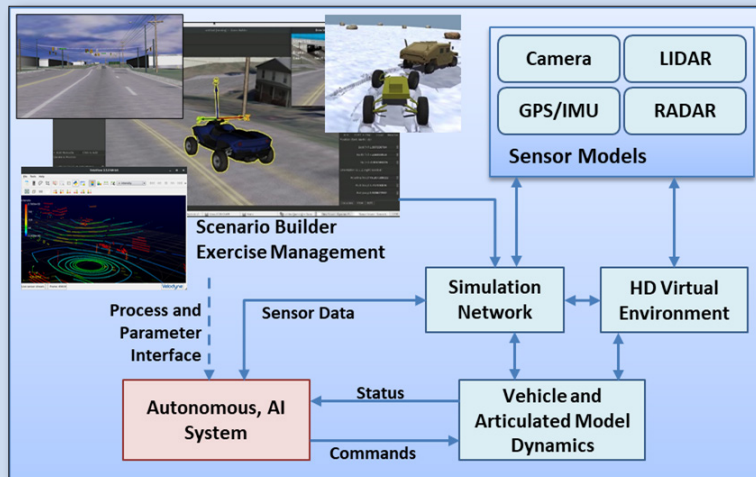
VxSIM - Virtual Exercise Framework
