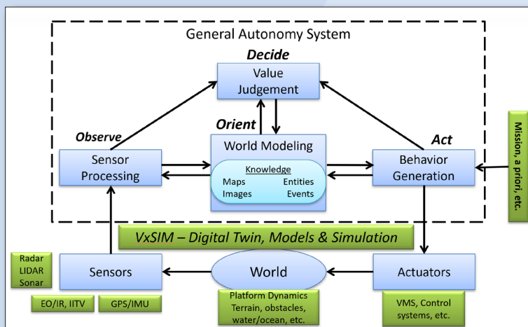
Real-Time simulation testing
